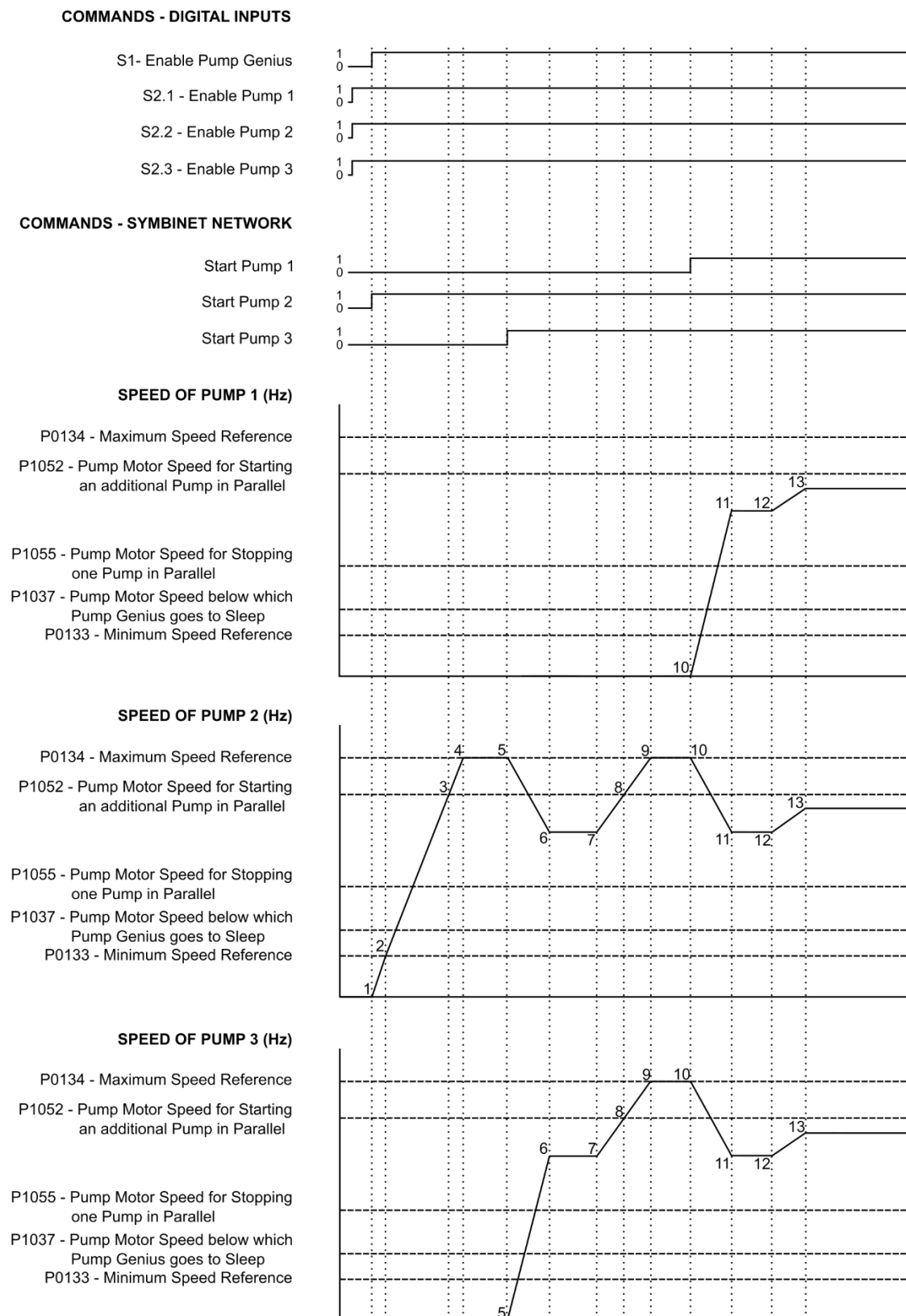
Figure 2.35 – Operation description of the Pump Genius Multiplex with three pumps in parallel
