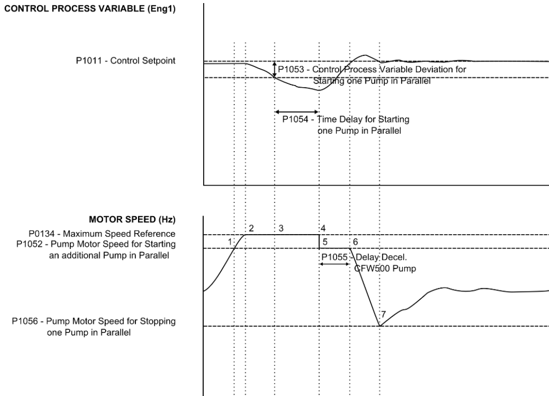
Figure 3.5 – Pump Genius operation for starting an additional pump in parallel
