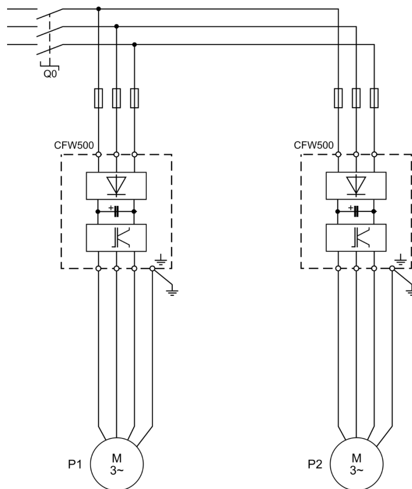
Figure 2.26 – Power connections of the Pump Genius Multiplex application with two pumps in parallel
