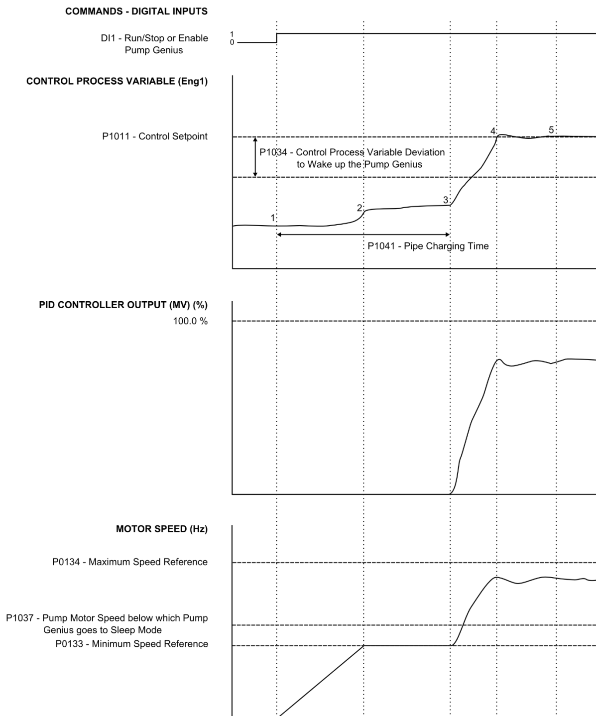
Figure 3.4 – Operation of the Pump Genius with pipe charging enabled
