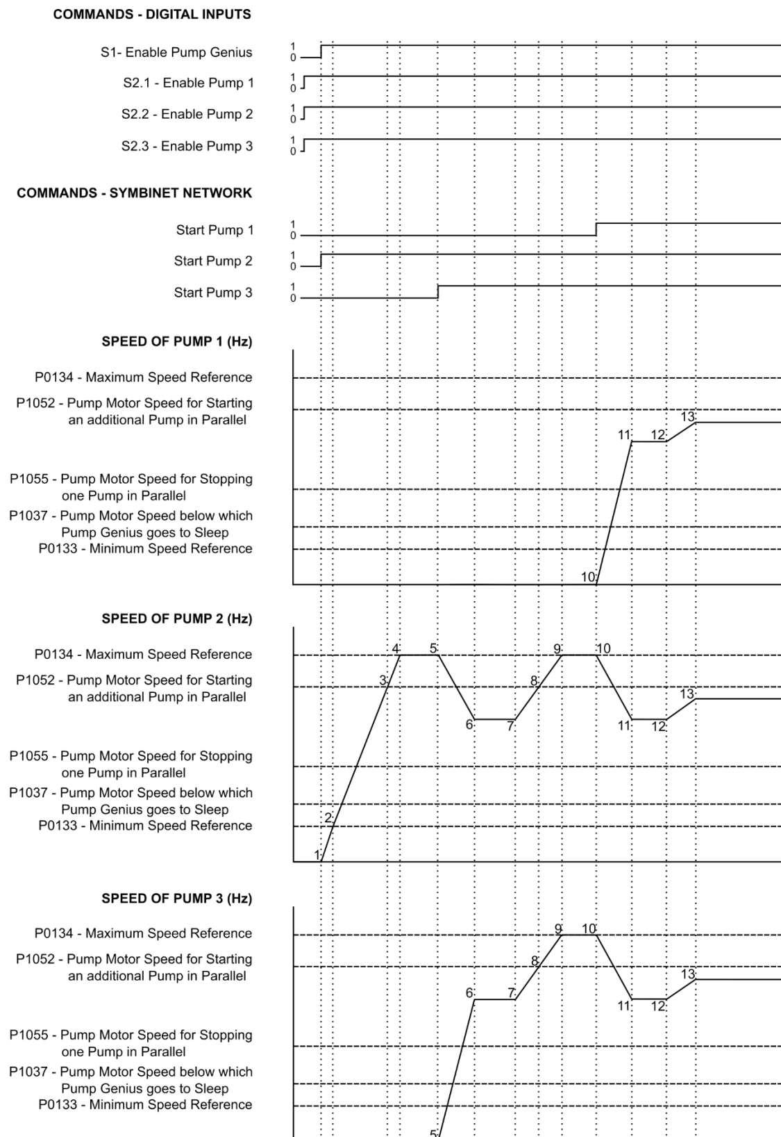
Figure 2.42 – Operation description of the Pump Genius with four pumps in parallel
