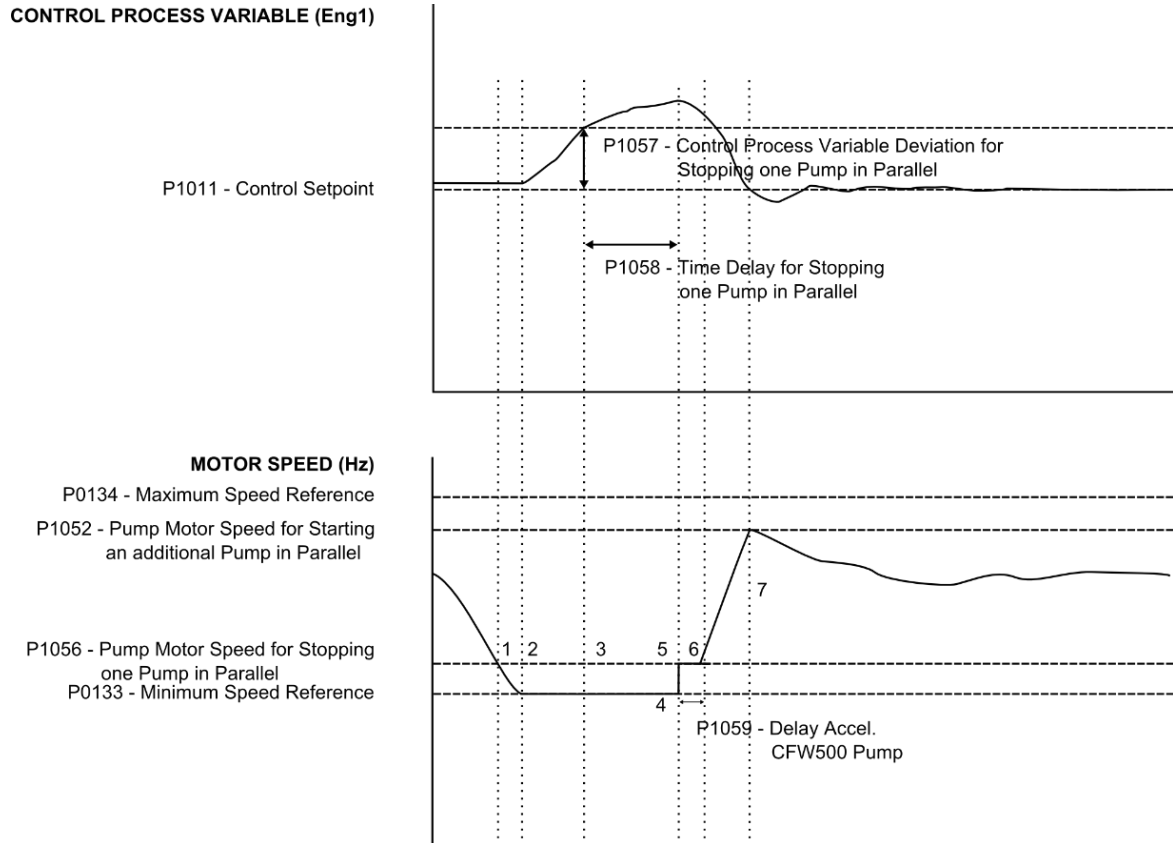
Figure 3.7 – Pump Genius operation for stop one pump in parallel
