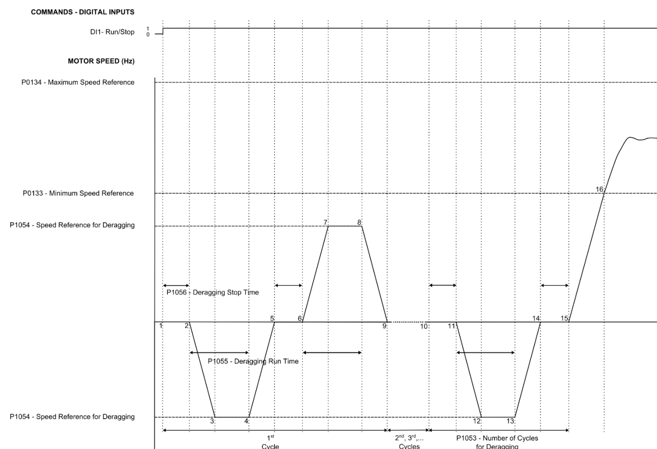
Figure 3.11 – Deragging pump operation with command to run the pump
