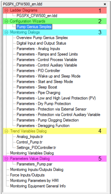
Figure 6.1 – Project Tree
