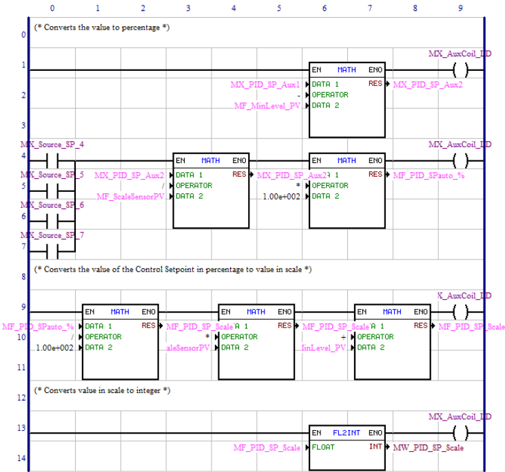
Figure 6.2 – Ladder Diagrams
